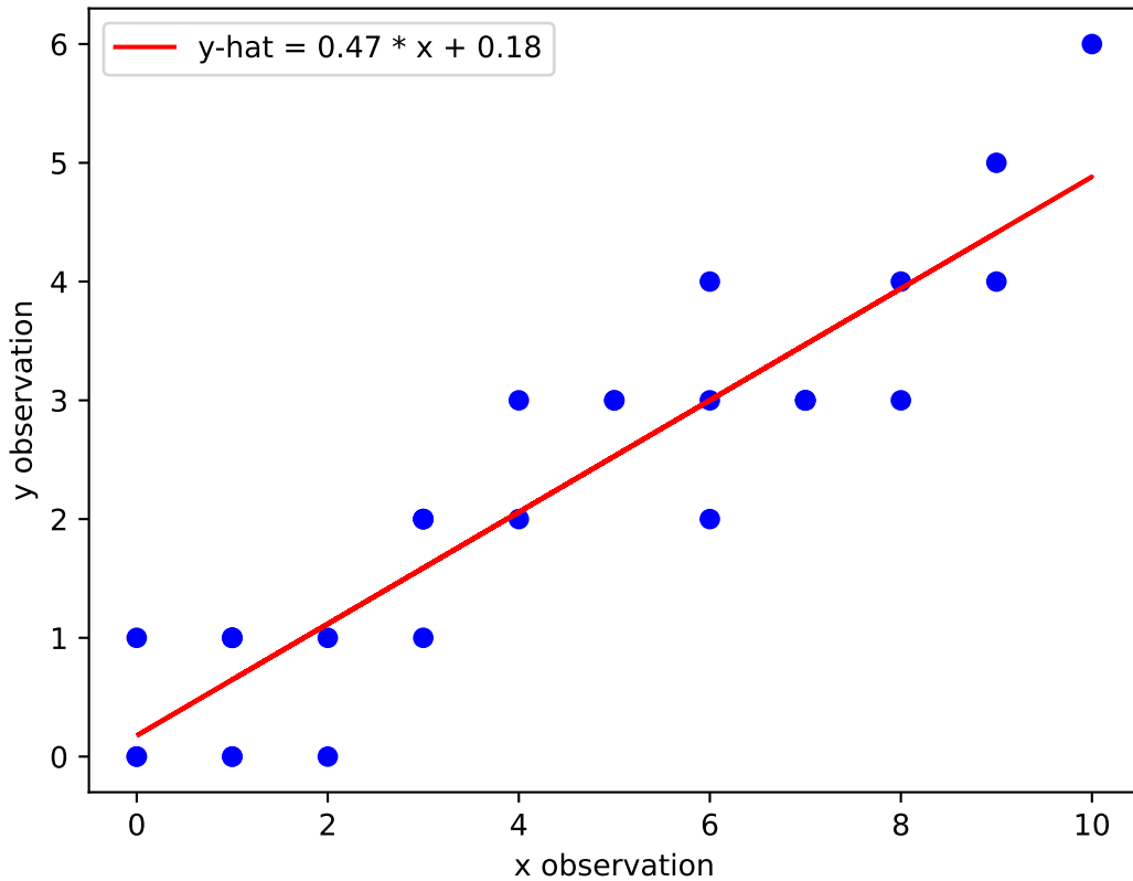
Scatterplot Example
