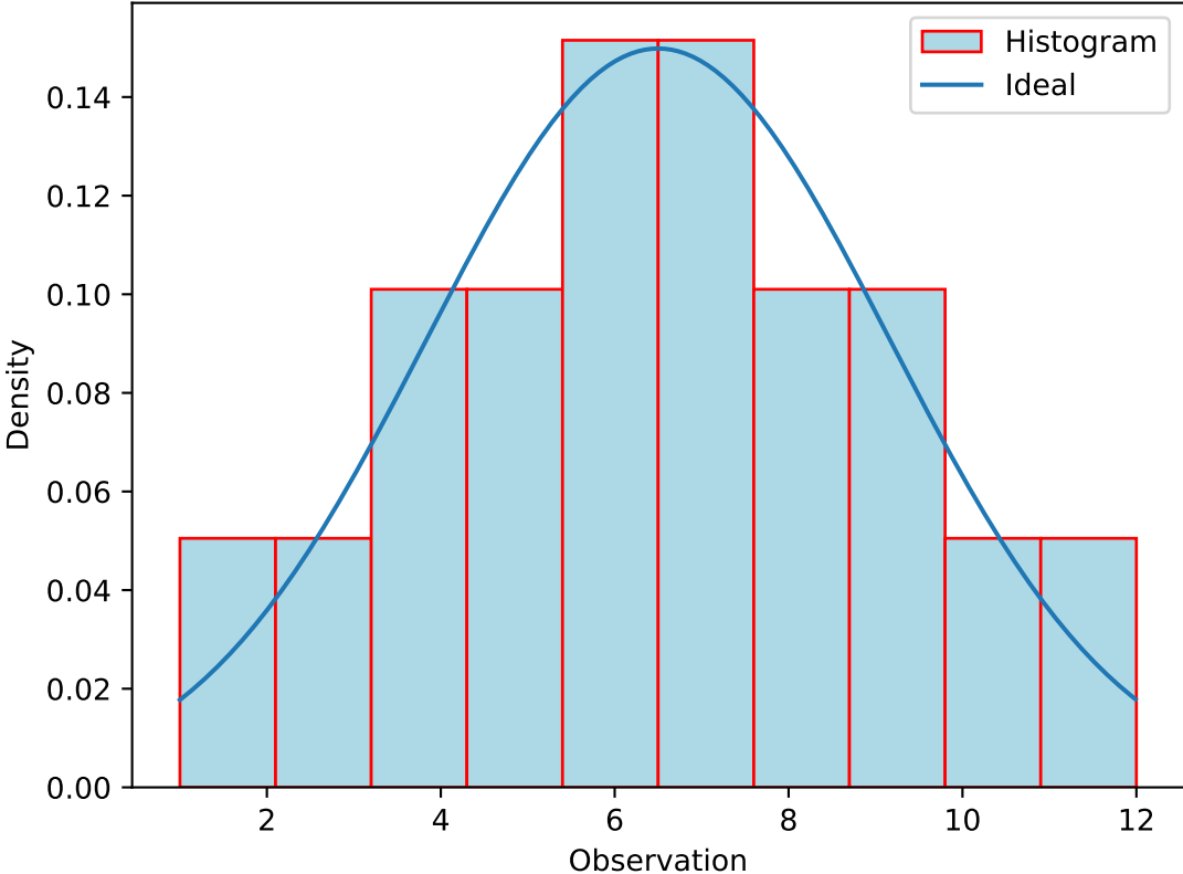
Sample vs. Ideal Distribution
